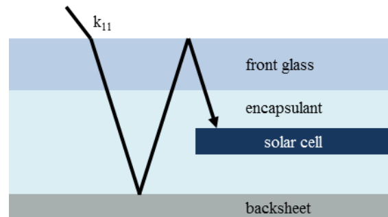
Figure 1: schematic drawing of backsheet reflection gains in modules with monofacial cells and opaque rear cover [13]
