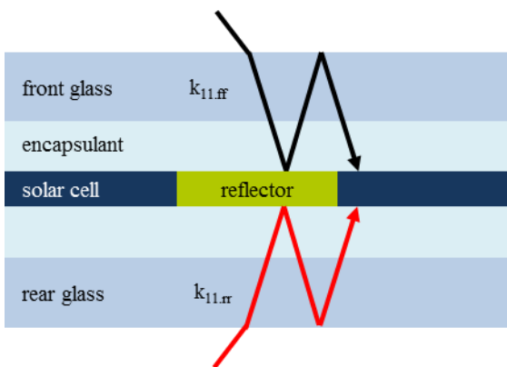
Figure 4: Schematic drawing of cover reflection gains in modules with bifacial cells, transparent rear cover and additional reflectors in the cell/string spacing area
